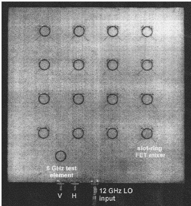
Fig. 10. A 2-D retrodirective array using ring slot antennas [74].
