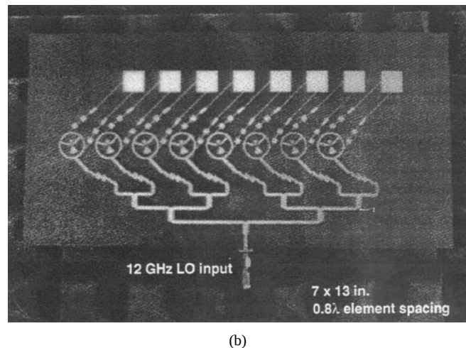
Fig. 9. (a) Heterodyne-phased scattering element. (b) Eight-element retrodirective array [72].
